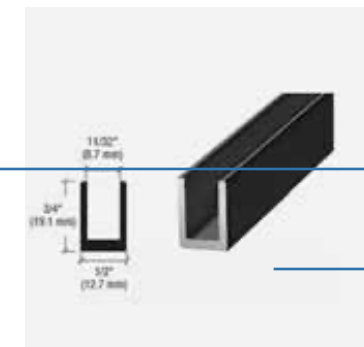
Vertical Aluminum U - Channel CRL SDCD516MBL Matte Black 5/16" Single Aluminum U-Channel
